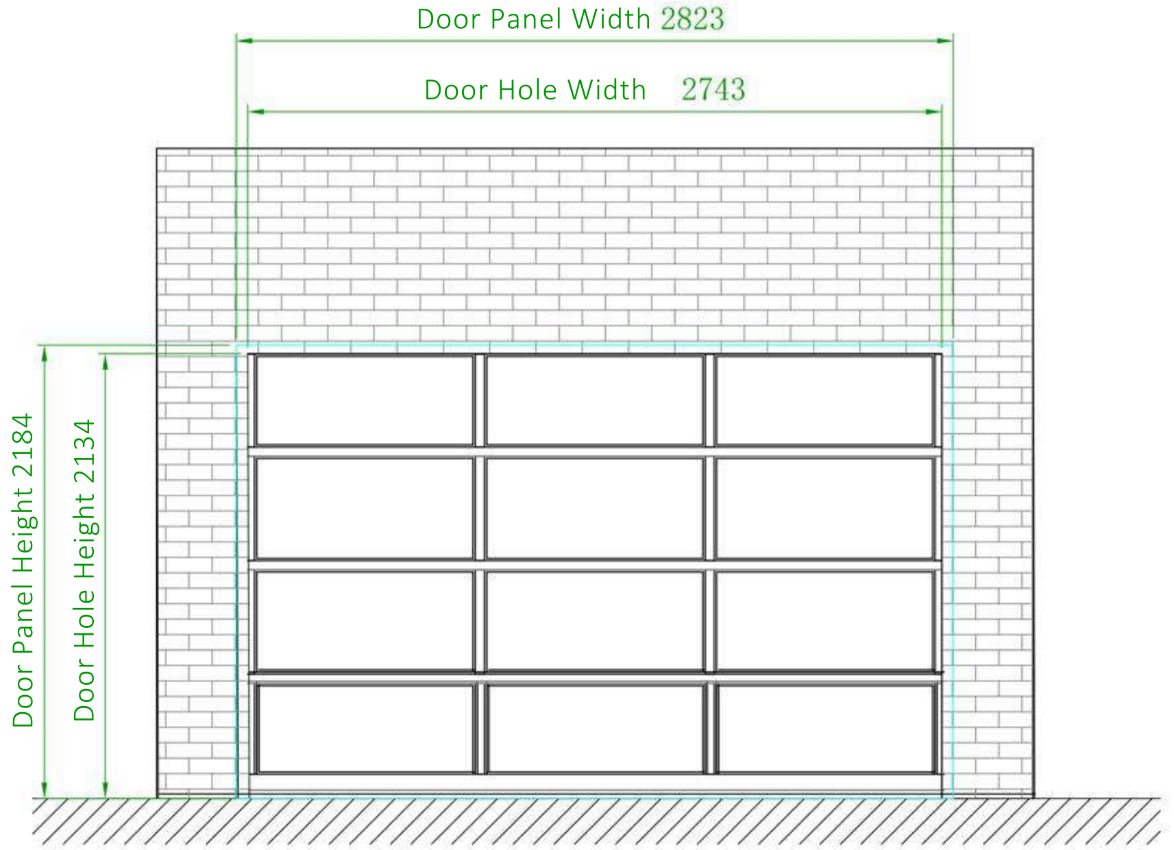
4X3 Aluminum Perspective Interior Front View
