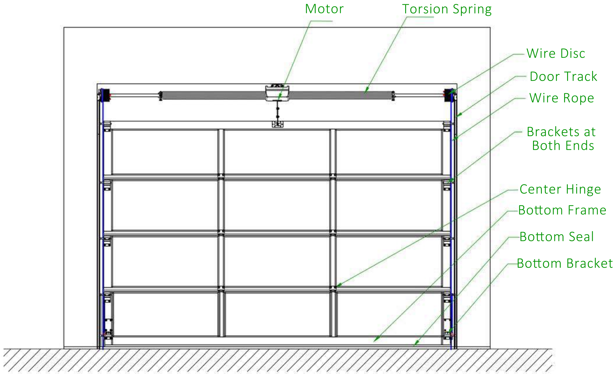
4X3 Aluminum Perspective Interior Rear View
