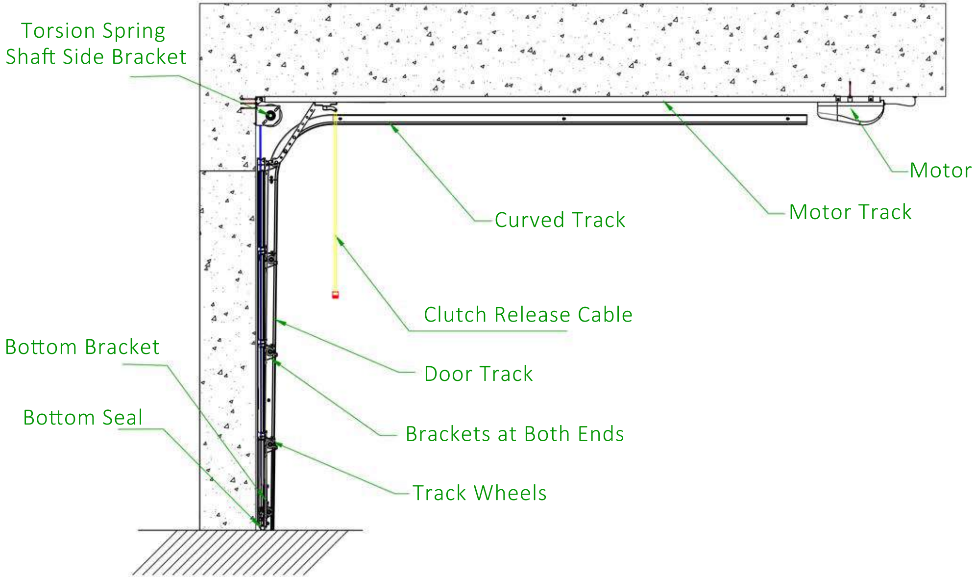
4X3 Aluminum Perspective Interior Side View
